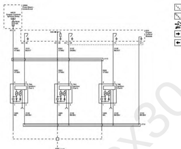
Ignition Controls - Ignition Coils 2, 4, and 6
