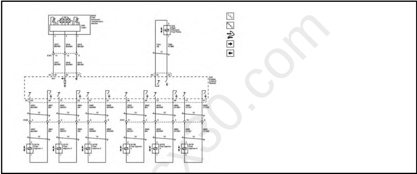
Fuel Controls - Fuel Pump Controls
